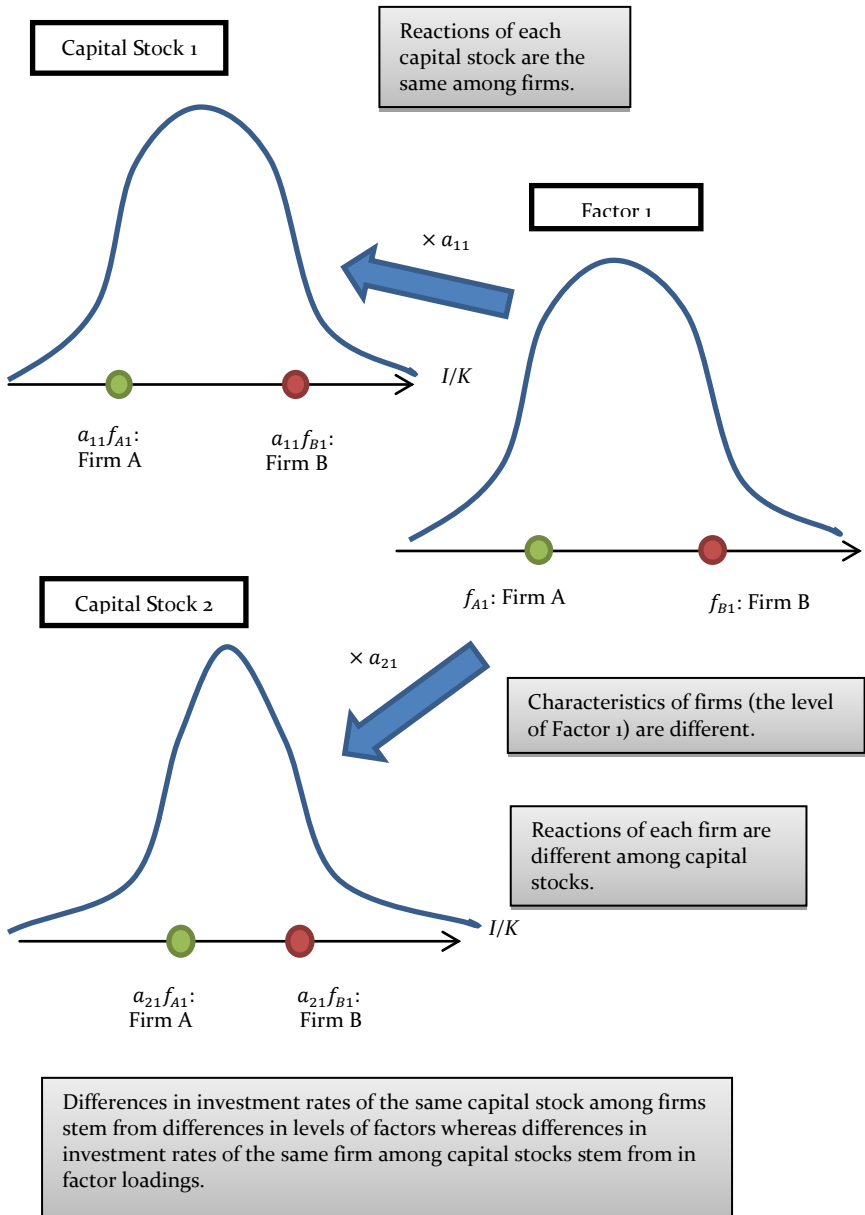
Figure 1: Image of Factor Analysis (1 Factor, 2 Capital Stocks)
